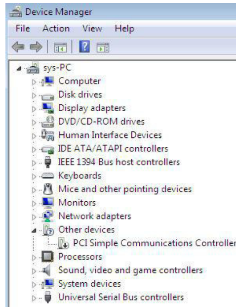
Fig 2.16 Device Manager
