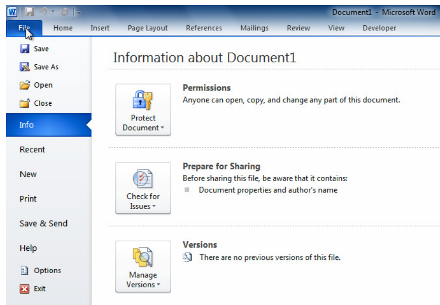
Fig 3.8 Backstage View
