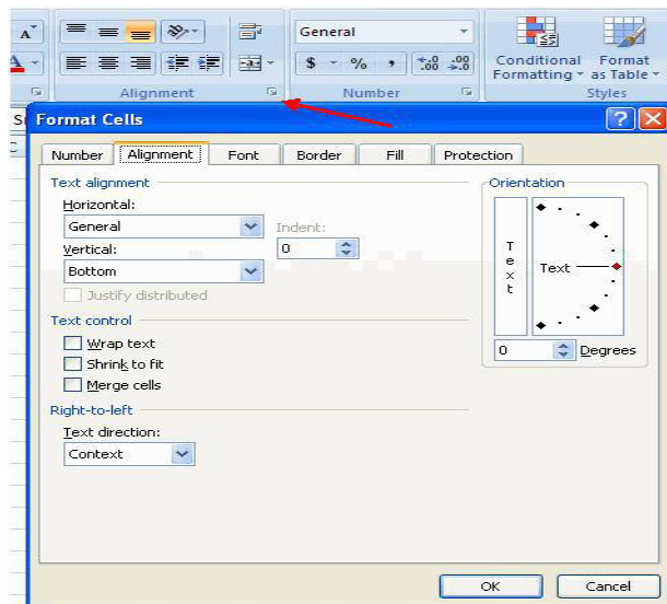
Fig. 4.43 Formatting Cells
