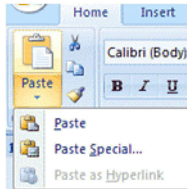
Fig 3.22 Paste button
