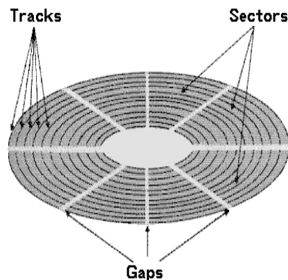
Fig 1.7 magnetic disc
