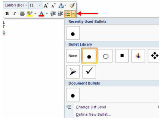
Fig 3.81 formatting list
