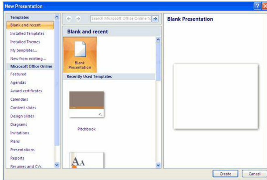
Fig 5.9 New Presentation
