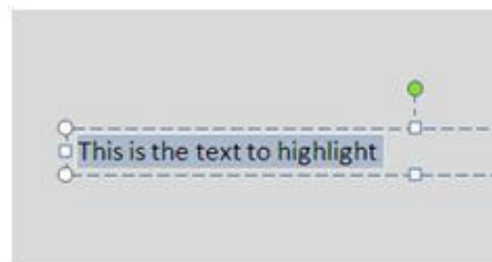
Fig 5.22 Text box
