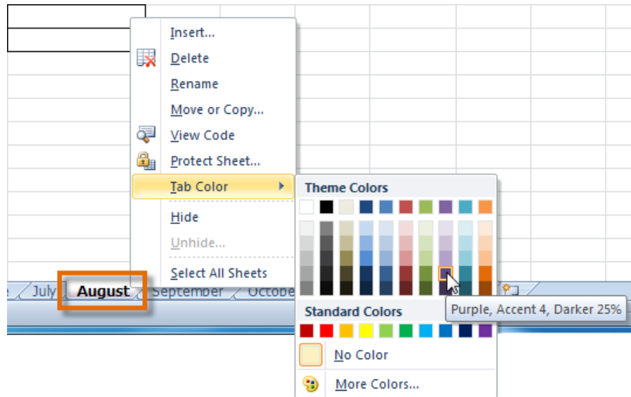
Fig 4.16 moving color
