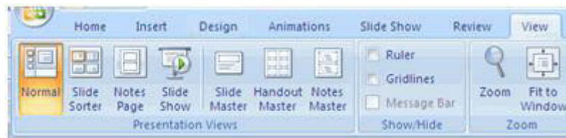
Fig 5.8 Slide Views
